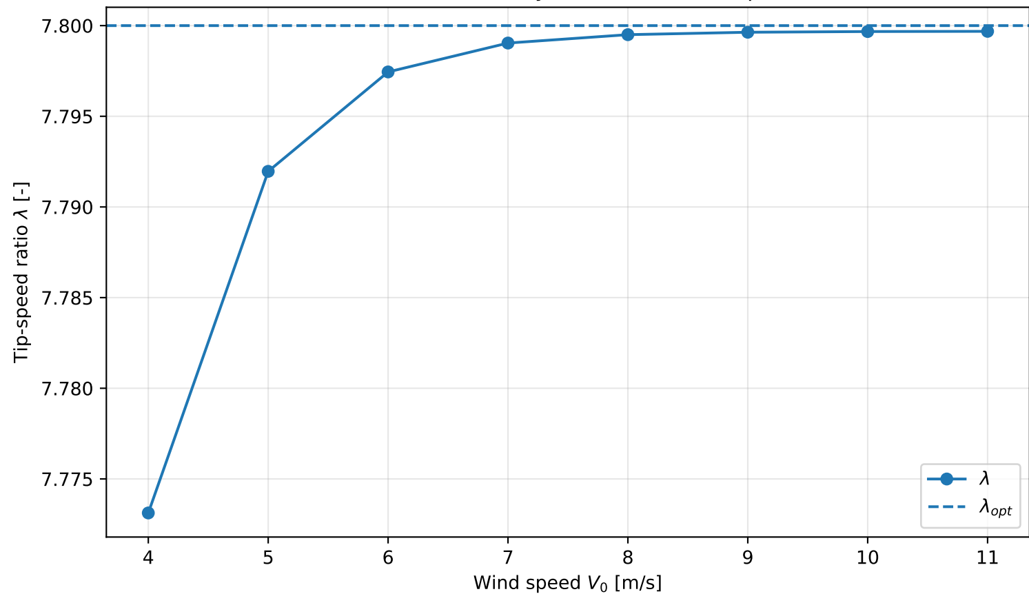
Below-rated steady lambda vs wind speed
